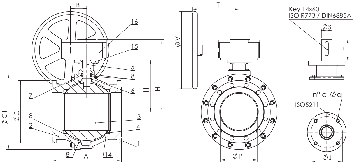
B2.0/B2.1 - DN 250
